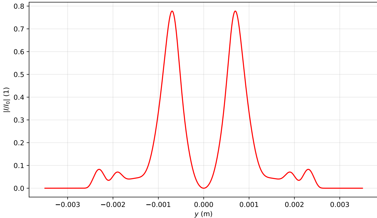
Intensity profile I(x=0, y, z=3.423)/I_0 , \text{Pin}=5.0\text{Pcr} , artificial time
